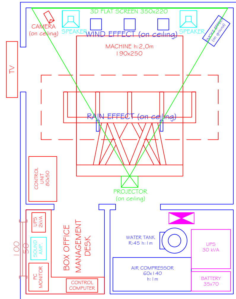
MACHINE LAYOUT PLAN
